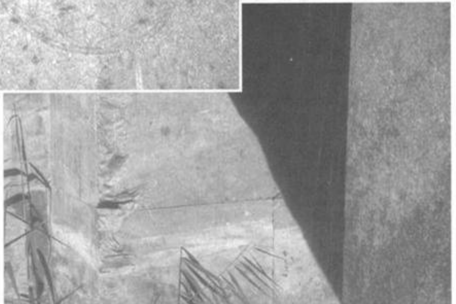
Fig. 2-14 Signo Copto
